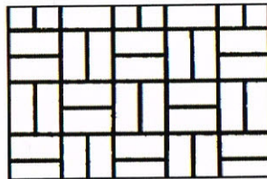
BASKET WEAVE Brick Size 200 x 90mm
